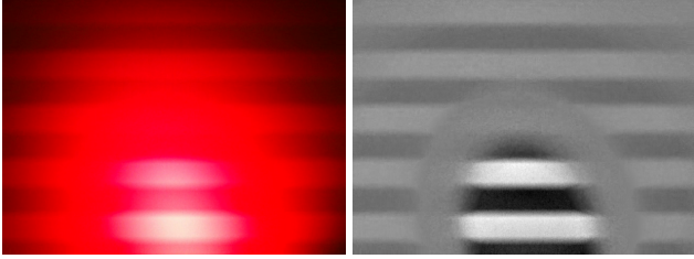
Figure 2. Calibration of a rolling-shutter camera. Left: Image of a flashing LED used for calibration of the readout time. Right: Corresponding image after subtraction of the temporal average.
