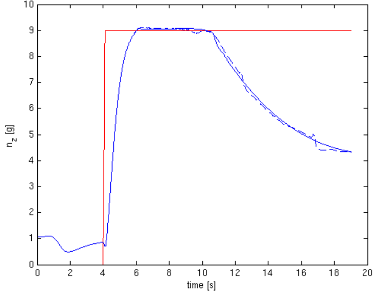
Figure 6. Load factor response for the command governor with model error estimator (dashed blue line) and without the model error estimator (solid blue line).
