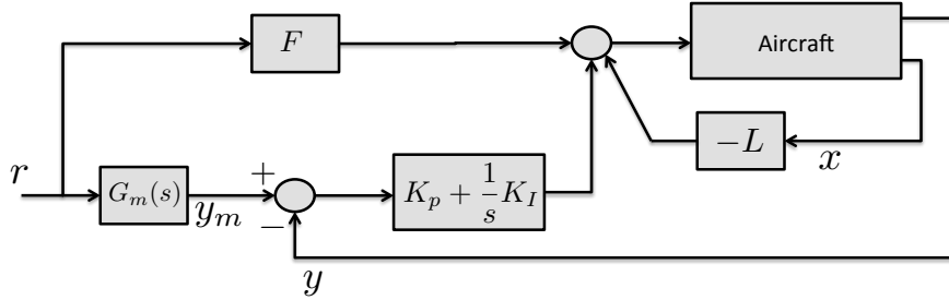
Figure 2. The nominal controller of the ARES model.
