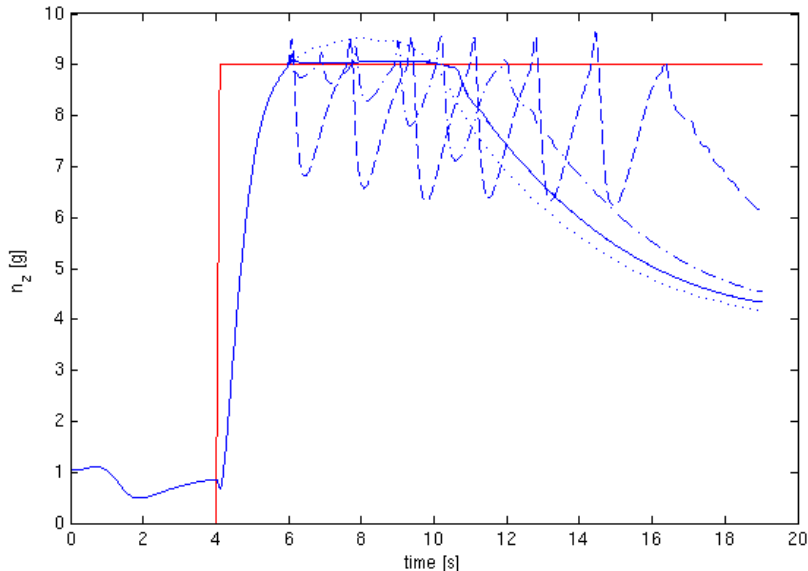
Figure 8. The normal load factor response of the closed loop system for different weight combinations in the command governor objective function. The solid blue line is the weights \beta_1 = 0.01 , \beta_2 = 0.1 . The dashed and dash-dotted lines are \beta_1 = 0.001 , \beta_2 = 0.01 and \beta_1 = 0.01 , \beta_2 = 0.001 respectively and the dotted line are the tuning with \beta_1 = 10 , \beta_2 = 100 . The red line is the pilot commanded load factor.
