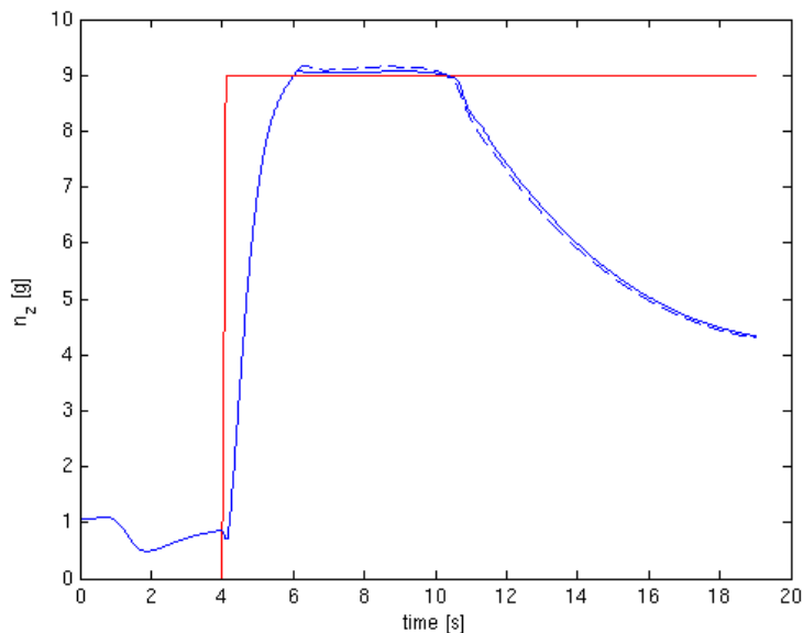
Figure 5. Load factor response for the command governor with Euler discretization of the response model (solid blue line) and with the Tustin discretization (dashed blue line). Red line is pilot commanded load factor.
