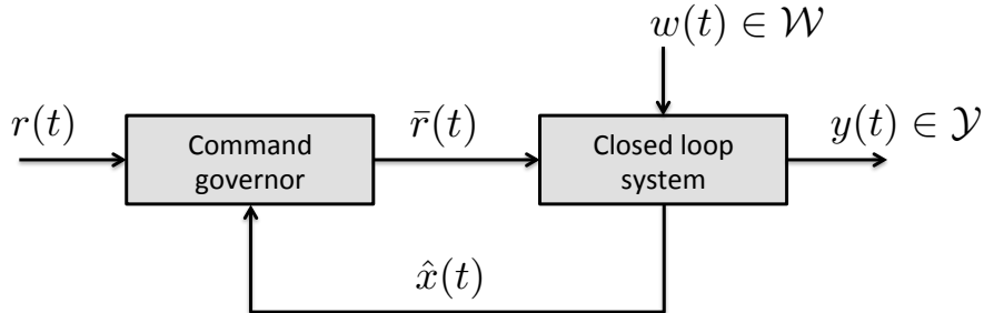
Figure 3. The reference governor general structure.
